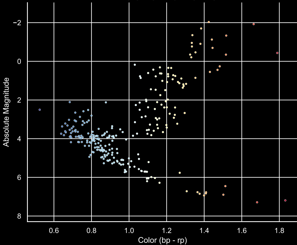
GALAH Hertzsprung-Russell Diagram Field [41] Ra [324.51] Dec [-56.06]
