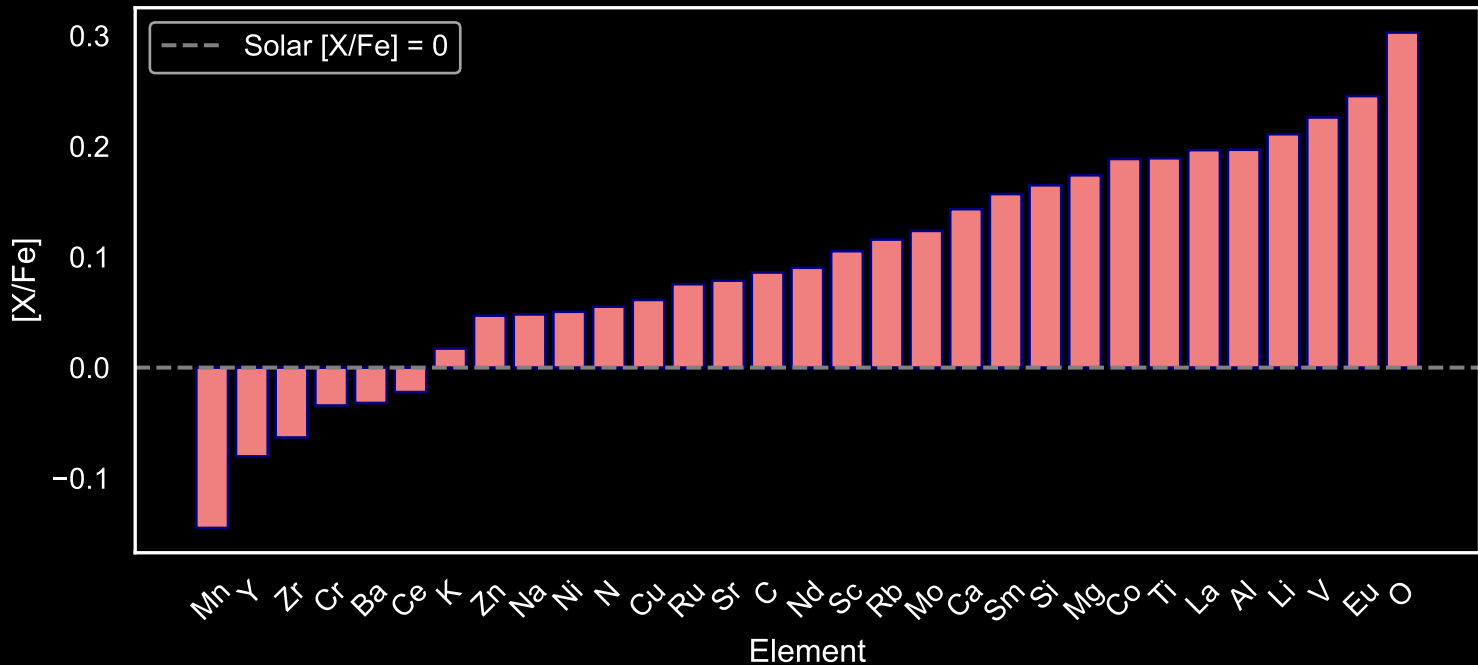
Abundance Pattern for GALAH Red Giants: Star Field [41] (N=75)
